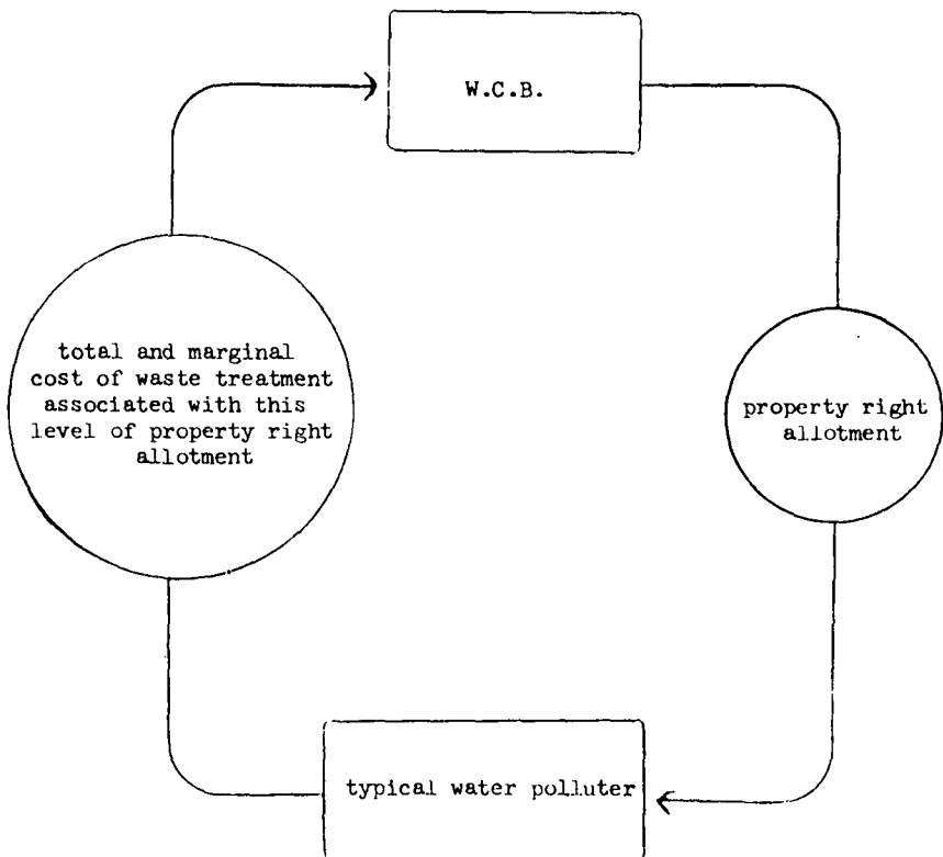
Portrayal of the communication linkage in a typical iteration of the allocation algorithm.
